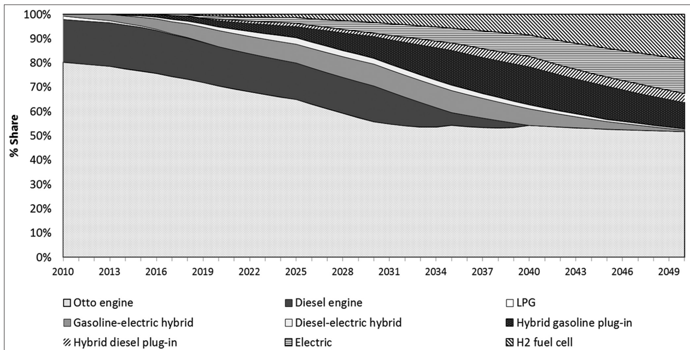
Figure 8: Annual light-duty vehicles sales, blue map scenario to Ecuador (2010–2050)
