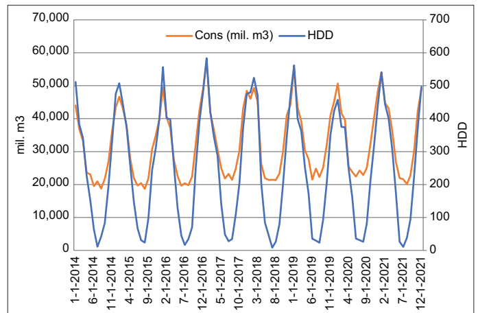
Figure 2: Correlation of natural gas consumption and HDD
