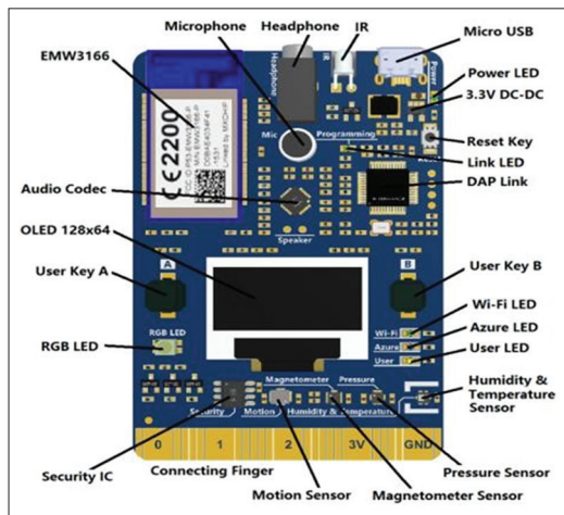
Figure 13: Sensor node
